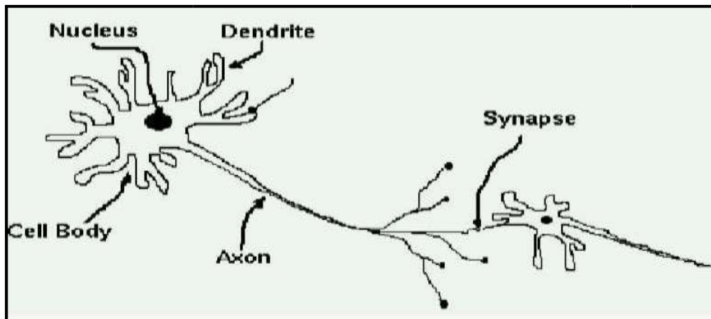
Fig.2.A Biological Neuron
