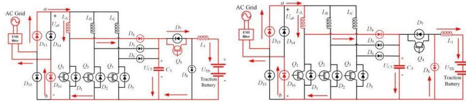
Traction battery charged by the grid. (a) Stage 1. (b) Stage 2. (c) Stage
